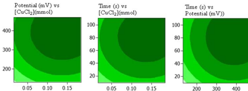
Fig. 2. Contour plots of variables involving in CCD used for optimization of electrodeposition procedure of CuNPs.
