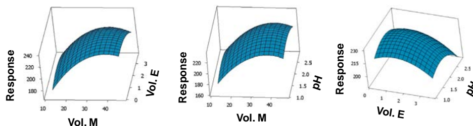
Fig. 4. Response surface obtained using central composite design for final optimization of variables related to pre-concentration/elution of ZIN.
