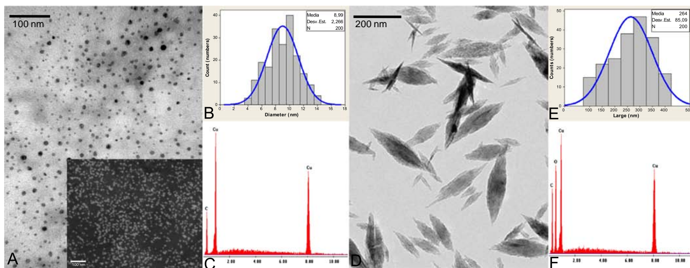
Fig. 1. Characterization of CuNPs and CuONPs. (A) Morphology of CuNPs was investigated by TEM and SEM, (B) CuNPs size distribution histogram and the fitted normal distribution curve, (C) elemental composition of CuNPs was determined by EDS, (D) morphology of CuONPs was investigated by TEM, (E) CuONPs size distribution histogram and the fitted normal distribution curve and (F) elemental composition of CuONPs was determined by EDS.
