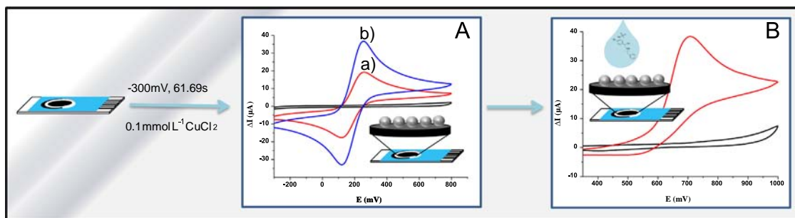
Scheme 2. (A) Electrochemical characterization by cyclic voltammogram was performed in 1 \text{ mmol L}^{-1} \text{ K}_3[\text{Fe}(\text{CN})_6]/\text{K}_4[\text{Fe}(\text{CN})_6] in 0.1 \text{ mol L}^{-1} \text{ KCl} . Cyclic voltammograms on (a) unmodified SPCE and (b) CuNPs/SPCE. (B) Electrochemical behavior of 1 \text{ mmol L}^{-1} \text{ ZIN} in 0.1 \text{ mol L}^{-1} \text{ glycine} (scan rate: 75 \text{ mV s}^{-1} ; T=25 \pm 1 \text{ }^\circ\text{C} ).
