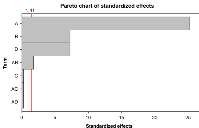
Fig. 3. Pareto chart obtained from 2^{4-1} fractional factorial design used as first optimization approach for variables related to pre-concentration/elution of ZIN. (A) Sample volume, (B) eluent volume, (C) eluent concentration, and (D) pH of eluent.
