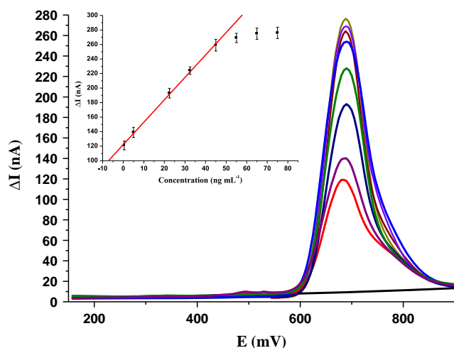
Fig. 5. Square wave voltammetry for ZIN detection. Calibration curve showed a linear range between 0.5 and 45 ng mL -1 of ZIN with a LOD of 0.16 ng mL -1 .
